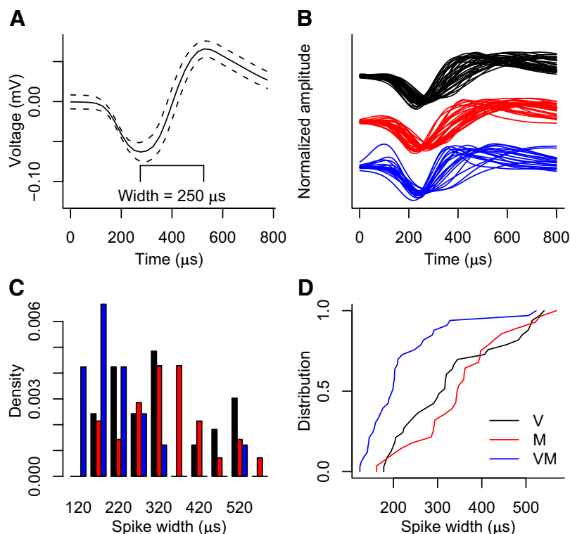
FIG. 2. Spike width by neuron type. A : mean (—) and mean \pm SD (---) spike waveforms from a representative visuomovement neuron. B : all mean, normalized spike waveforms for visual (V, black), movement (M, red) and visuomovement (VM, blue) neurons. C : histogram of spike widths for each type of neuron. D : cumulative distribution of spike widths for each type of neuron.
