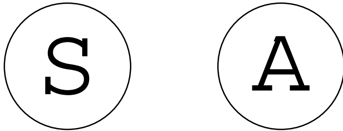
Fig. 1b) A drawing reproduced from Wheatstone's monograph (Figure 25) showing a pair of dissimilar "half-images" that inspired Wheatstone rather detailed descriptions of binocular rivalry.
