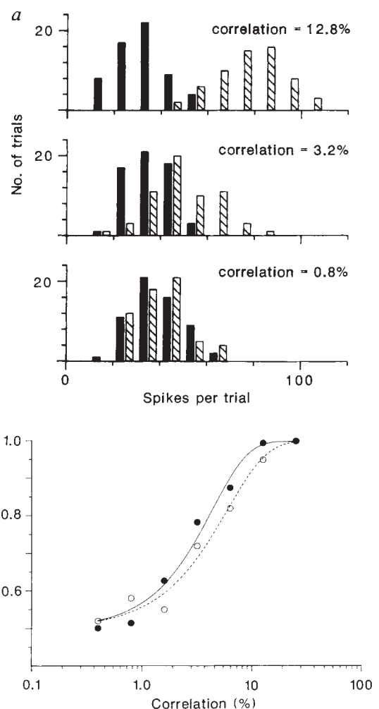
FIG. 1 Physiological and psychophysical data obtained simultaneously from a rhesus monkey. a , The responses of a directionally selective MT neuron at three different motion correlations spanning physiological threshold. The hatched bars represent responses to motion in the neuron's preferred direction; the solid bars indicate responses to motion in the null direction (180° opposite to the preferred). Sixty trials were performed in each direction for each of the three correlation levels. Response distributions for a range of correlation levels were used to compute a 'neurometric' function that characterized the neuron's sensitivity to the motion signal and could be compared with the psychometric function computed from the monkey's behavioural responses. b , Comparison of simultaneously recorded psychometric and neurometric functions. Psychophysical performance of the monkey, ○; performance of the neuron, ●. Psychophysical performance at each correlation is given by the proportion of trials on which the monkey correctly identified the direction of motion. Neuronal performance is calculated from distributions of responses like those in Fig. 1a, using a signal-detection method described in the text. The physiological and psychophysical data form similar curves, but the data for the neuron lie to the left of the data for the monkey, meaning that the neuron was somewhat more sensitive than the monkey. We fit the data with smooth functions of the form introduced to psychophysics by Quick 12 . Threshold, defined as the correlation for which the direction of motion was identified correctly on 82% of the trials, was 6.1% for the monkey and 4.4% for the neuron.
