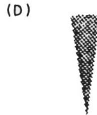
99% confidence interval for population vector
